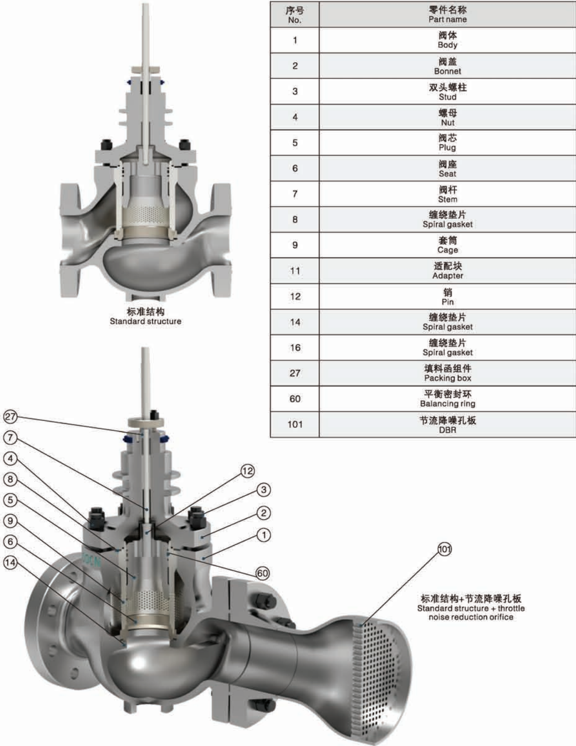
◆图1 DC1624L/X低噪音与特殊低噪音套筒调节阀本体部结构图 Figure 1 Structure of dc1624l/X low noise and special low noise sleeve control valve body
