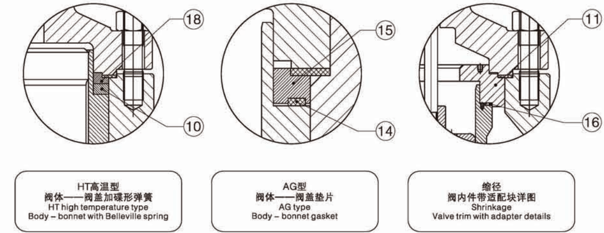
◆DC1624L/X特殊工况下可选结构 DC1624L/X optional structure under special working condition
